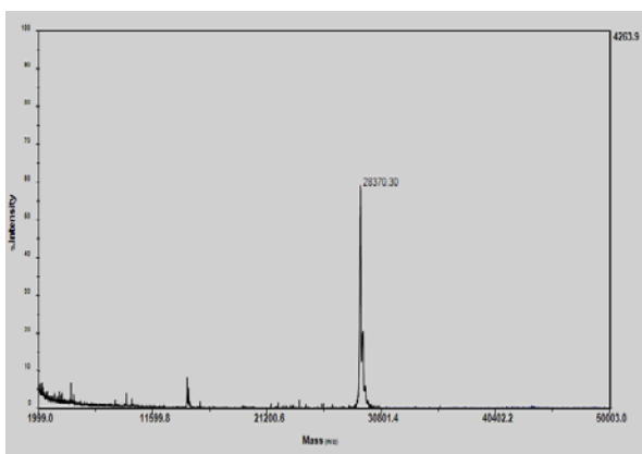
Fig. 3: MALDI/MS analysis of BGS-Haridrin
