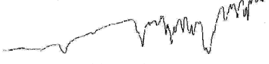
Fig-5 c) FT-IR of PMPEG 6000
