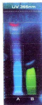
Fig.1: HPTLC analysis of methanolic extracts of Lantana camara (Linn.) Fruit
