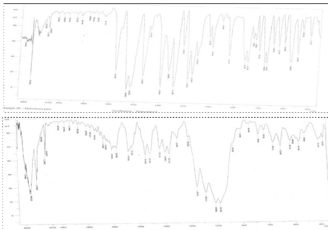
Fig. 3: Fourier transform infrared spectra of A: Pure Meloxicam B: Meloxicam tablet (From top to bottom)
