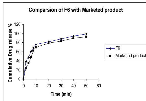
Fig. 2: Comparison of In-vitro release profile of formulation F6 with marketed sample
