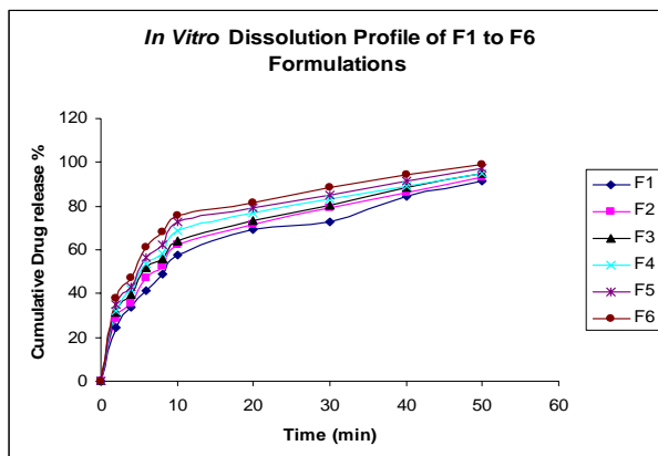
Fig. 1: Comparison of In-vitro release profile of Meloxicam from formulations F-1 to F-6
