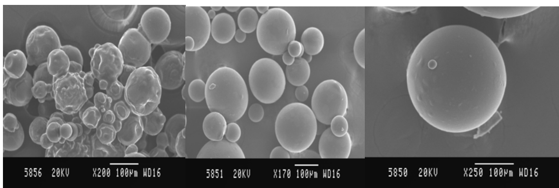
Fig. 2: Scanning Electron Micrographs (SEM) of Trimetazidine hydrochloride microspheres (a) Microspheres prepared with 1:1 drug/polymer ratio, (b) Microspheres prepared with 1:2 drug/polymer ratio, (c) Microspheres prepared with 1:3 drug/polymer ratio
