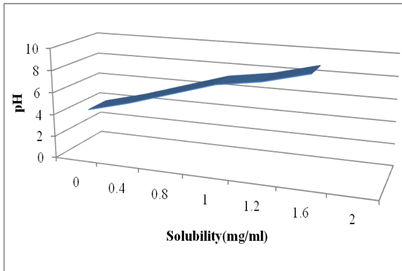
Fig. 3: Effect of pH on drug solubility
