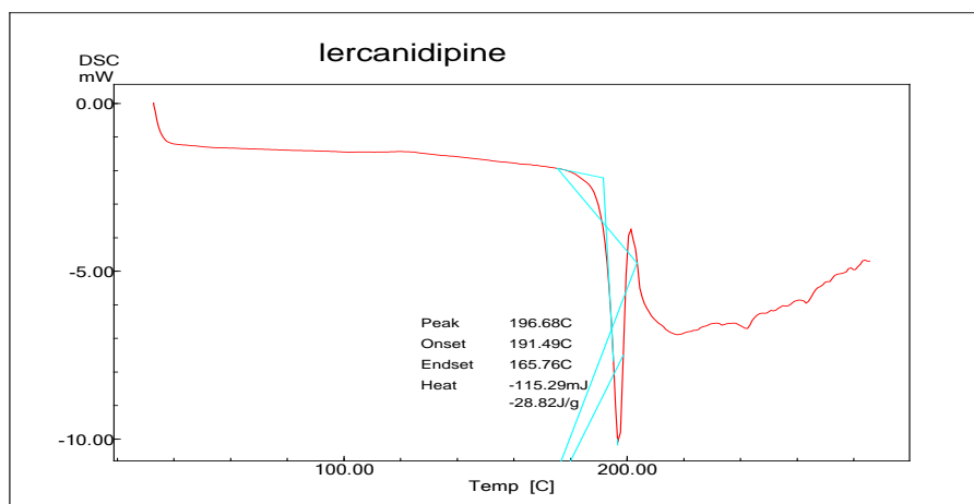
Fig. 2: DSC thermogram of Lercanidipine HCl
