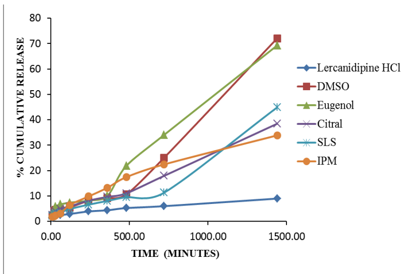
Fig. 4: Preformulation screening data of drug with various enhancers
