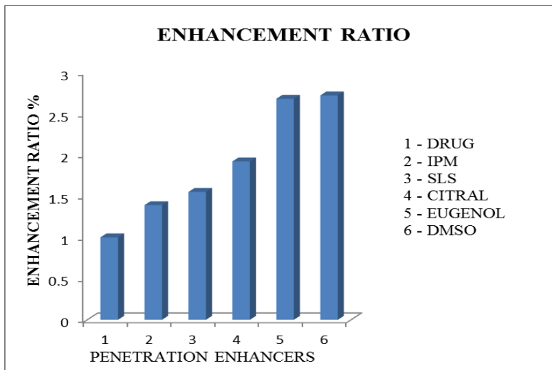
Fig. 5: Bar graph showing enhancement ratio of Lercanidipine Hcl with different penetration enhancers (n = 3)
