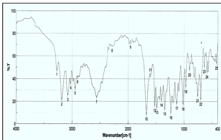
Fig. 1: FTIR spectra of Lercanidipine HCl
