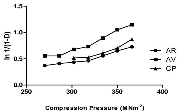
Fig. 1: Heckel plots for EVG compacts produced using selected diluents and PVP (5%w/v) as binder. Points refer to mean \pm SD values ( n = 3 )
