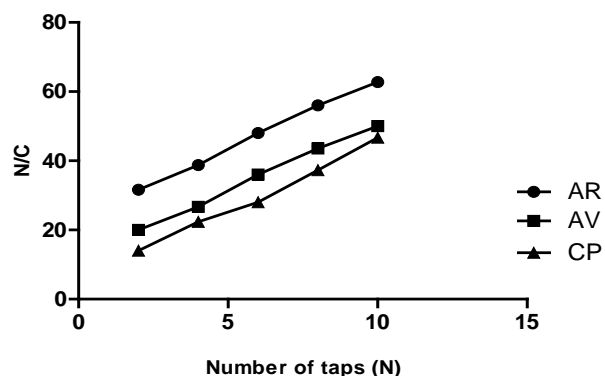
Fig. 2: Kawakita plots for EVG compacts produced using selected diluents and PVP (5%w/v) used as binder. Points refer to mean ± SD values (n = 3)
