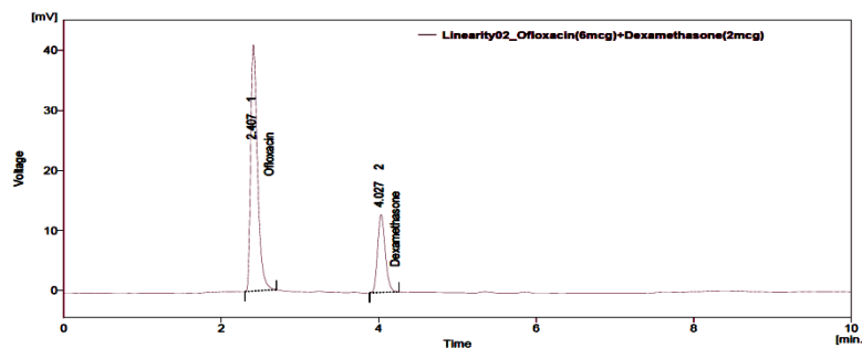
Fig. 2: Typical chromatogram for the standard solution of OFN and DSP
