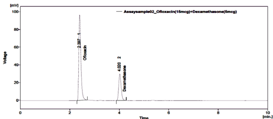
Fig. 3: Typical chromatogram for the sample solution of OFN and DSP
