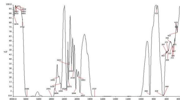
Fig. 7b: FTIR spectrum of (Coumarin-1 + \beta CD) complex
