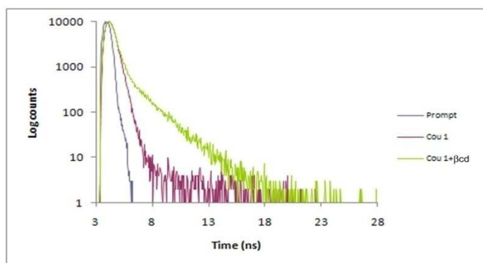
Fig. 6. Fluorescence decay curves of coumarin-1 and the inclusion complex of cou-1 with \beta CD
