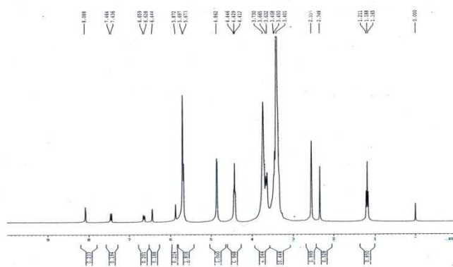
Fig. 8c: 1 H NMR spectrum of (Coumarin-1 + βCD) complex
