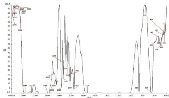
Fig. 7a: FTIR spectrum of Coumarin-1
