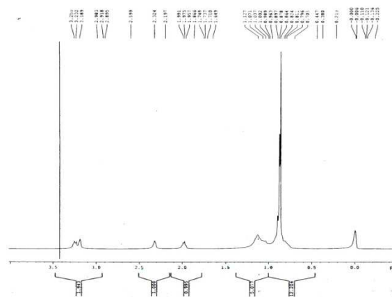
Fig. 8b: 1 H NMR spectrum of βCD
