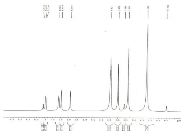
Fig. 8a: 1 H NMR spectrum of Coumarin-1
