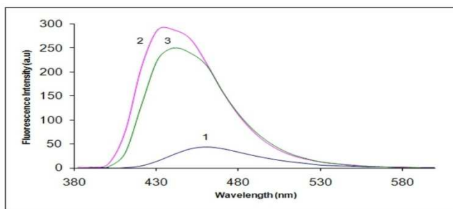
Fig. 1. Fluorescence spectra of Coumarin - 1 in different solvents 1. Water, 2. DMF, 3. DMSO
