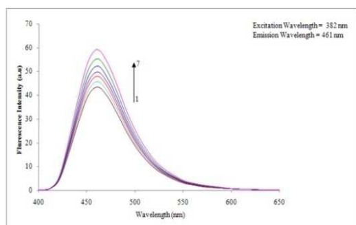
Fig. 3a. Fluorescence spectra of Coumarin - 1 in different \beta CD concentrations (mol dm -3 ) in water. (1) 0, (2) 0.002, (3) 0.004, (4) 0.006, (5) 0.008, (6) 0.010, (7) 0.012
