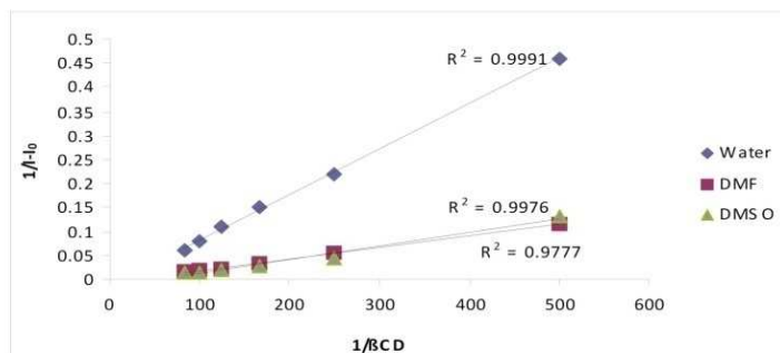
Fig. 5: Plot of \left(\frac{1}{I - I_0}\right) versus \left(\frac{1}{\beta - CD}\right) for Coumarin-1
