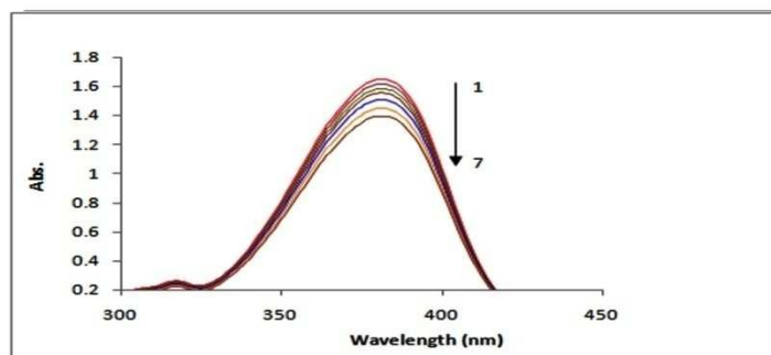
Fig. 2. Absorption spectra of Coumarin - 1 in different \beta CD concentrations (mol dm -3 ) in water. (1) 0, (2) 0.002, (3) 0.004, (4) 0.006, (5) 0.008, (6) 0.010, (7) 0.012
