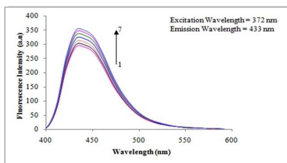
Fig. 3b. Fluorescence spectra of Coumarin - 1 in different \beta CD concentrations (mol dm -3 ) in DMF. (1) 0, (2) 0.002, (3) 0.004, (4) 0.006, (5) 0.008, (6) 0.010, (7) 0.012
