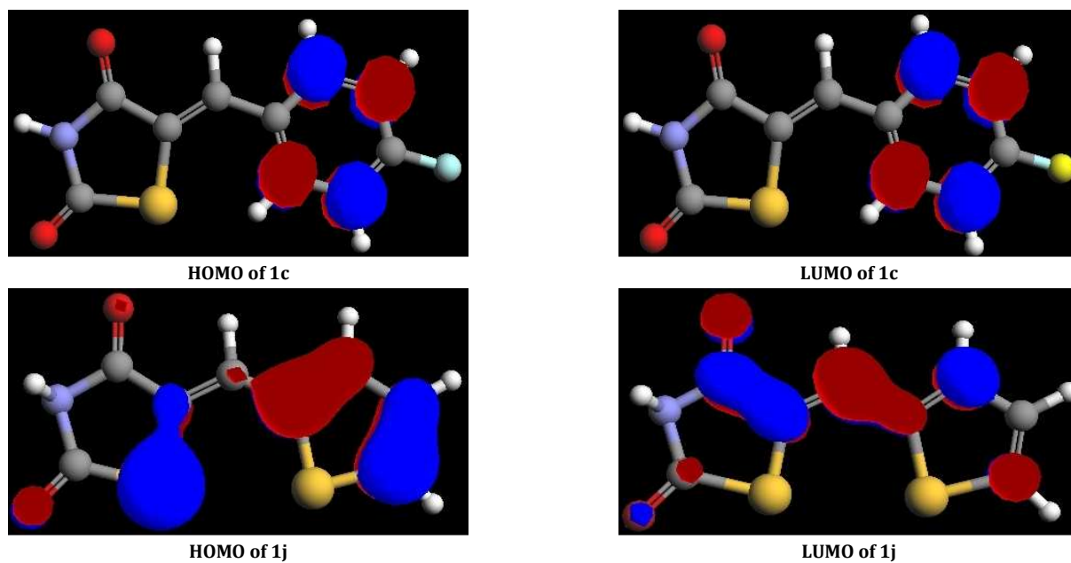
Fig. 1: Image showing HOMO and LUMO energies of compounds 1a, 1c and 1j
