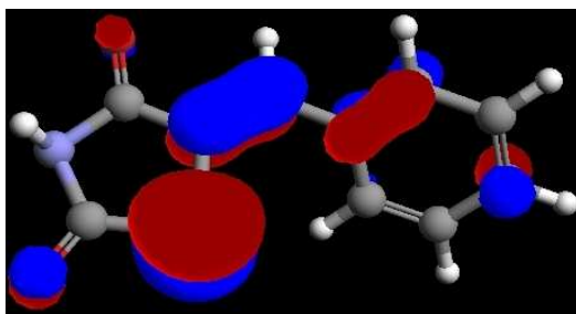
HOMO of 1a
