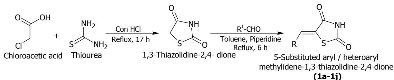
Scheme 1: The synthetic pathway for compounds 1a-1j
