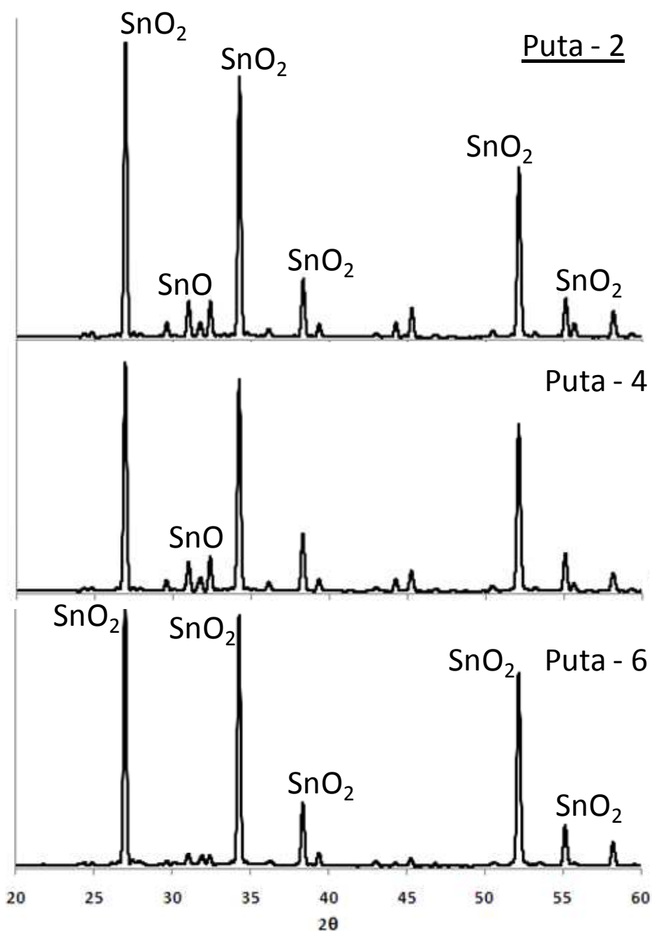
Fig. 6: X-ray diffractogram of intermediates after each puta showing the presence of \text{SnO}_2 and \text{SnO} phases. Note that \text{SnO} is absent in the final product
