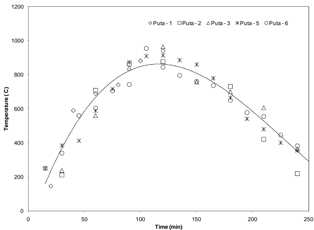
Fig. 3: Temperature profile during puta .
