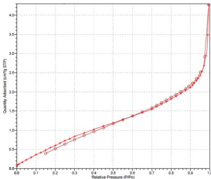
Fig. 5: BET isotherms of [A] intermediate after 1 st puta ; [B] final product.
