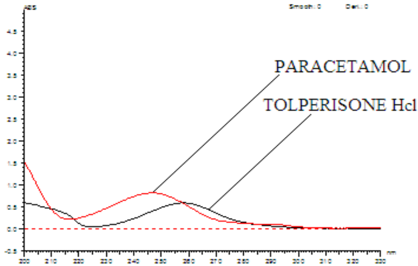
Fig. 2: Overlain spectrum of a mixture of standard Tolperisone HCl and Paracetamol
