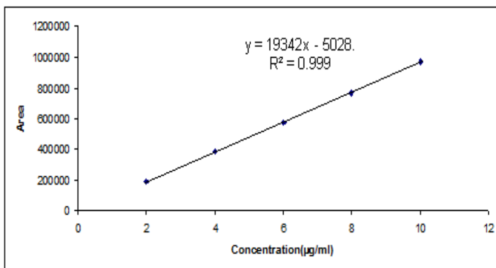
Fig. 4: Calibration curve of Paracetamol
