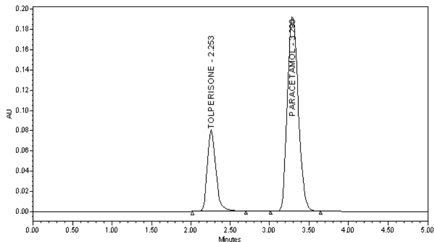
Fig. 3: Typical chromatogram of a mixture of standard Tolperisone HCl and Paracetamol
