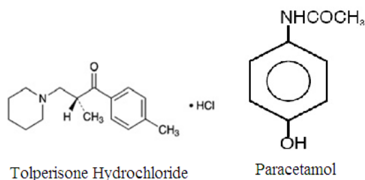
Fig. 1: Structure of Tolperisone Hydrochloride and Paracetamol
