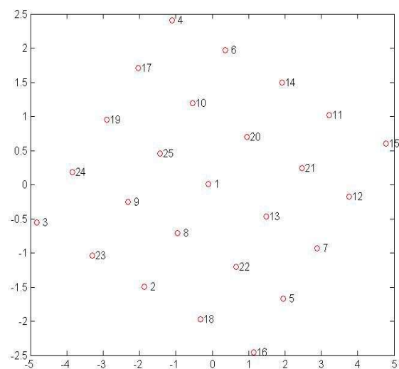
Fig. 2: The first two latent variables of the concentration matrix showing the relation between different samples.
