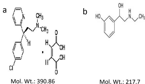
Fig. 1: Chemical Structure of (a) chlorpheniramine maleate and (b) etilefrine hydrochloride.
