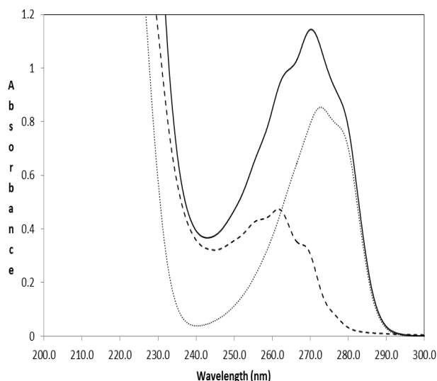
Fig. 3: Zero order absorption (0D) spectra of 30 µg ml -1 chlorpheniramine maleate (-----), 100 µg ml -1 etilefrinehydrochloride (-----) and mixture of both (——) using double distilled water as solvent.
