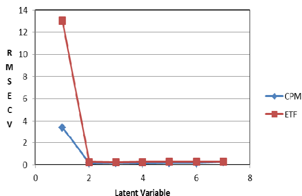
Fig. 4: RMSEC plot of the cross validation results of the calibration set as a function of the number of latent variables used to construct the PCR calibration.
