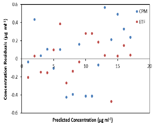
Fig. 6: Concentration residuals vs. predicted concentration of CPM and ETF using CLS (with non-zero intercept).
