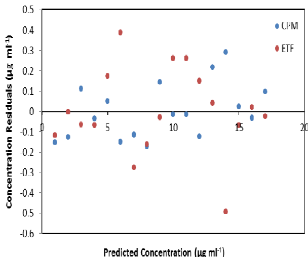
Fig. 7: Concentration residuals vs. predicted concentration of CPM and ETF using PCR.
