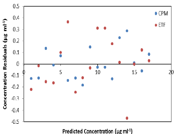
Fig. 8: Concentration residuals vs. predicted concentration of CPM and ETF using PLS.
