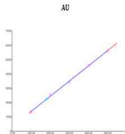
Fig. 1: Calibration curve of beta-sitosterol
