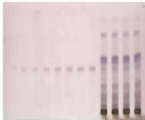
Fig. 2: High Performance Thin Layer Chromatography Separation of Standard β-sitosterol and Methanolic Extract of Dried leaves Powder of Holoptelea Integrifolia (Roxb.) planch .
