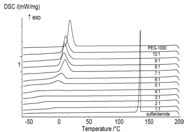
Fig. 3: DSC curves of initial samples of PEG-1000, sulfanilamide and their mixtures of varying composition (1-10:1) in dynamic atmosphere of argon 150 ml/min, in the temperature range of -60 to 200 °C (cooling). Cooling rate 10 °C/min
