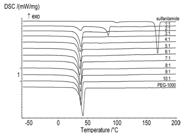
Fig. 2: DSC curves of initial samples of PEG-1000, sulfanilamide and their mixtures of varying composition (1-10:1) in dynamic atmosphere of argon 150 ml/min, in the temperature range of -60 to 200 °C (first heating). Heating rate 5 °C/min.
