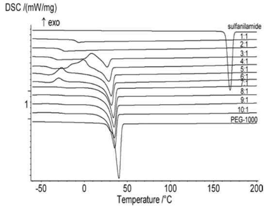
Fig. 4: DSC curves of initial samples of PEG-1000, sulfanilamide and their mixtures of varying composition (1-10:1) in dynamic atmosphere of argon 150 ml/min, in the temperature range of -60 to 200 °C (second heating). Heating rate 5 °C/min.
