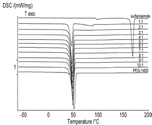
Fig. 5: DSC curves of initial samples of PEG-1400, sulfanilamide and their mixtures of varying composition (1-10:1) in dynamic atmosphere of argon 150 ml/min, in the temperature range of -60 to 200 °C (first heating). Heating rate 5 °C/min
