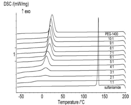
Fig. 6: DSC curves of initial samples of PEG-1400, sulfanilamide and their mixtures of varying composition (1-10:1) in dynamic atmosphere of argon 150 ml/min, in the temperature range of -60 to 200 °C (cooling). Cooling rate 10 °C/min.
