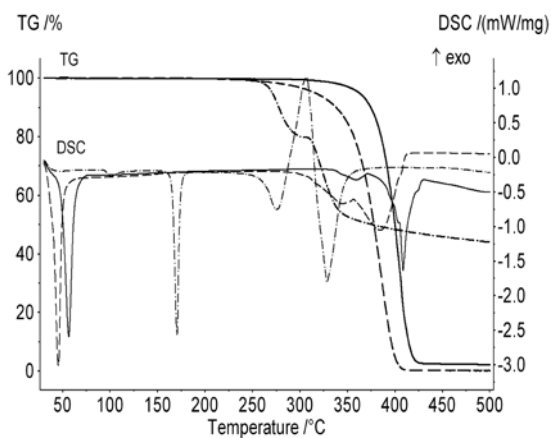
Fig. 1: TG/DSC curves of PEG-1000 (dashed line), PEG-1400 (solid lines) and sulfanilamide (dash and dot line) in dynamic atmosphere of argon 75 ml/min, in the temperature range 30 to 500 °C. Heating rate 5 °C/min.
