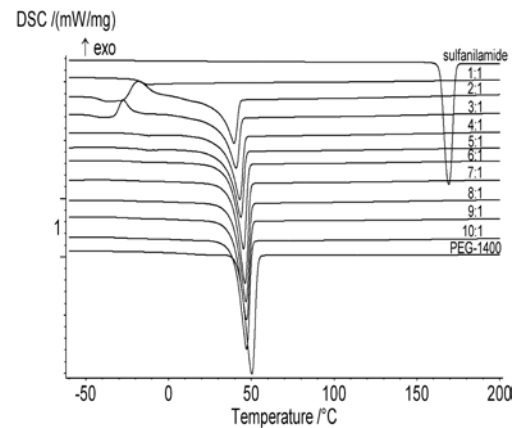
Fig. 7: DSC curves of initial samples of PEG-1400, sulfanilamide and their mixtures of varying composition (1-10:1) in dynamic atmosphere of argon 150 ml/min, in the temperature range of -60 to 200 °C (second heating). Heating rate 5 °C/min.
