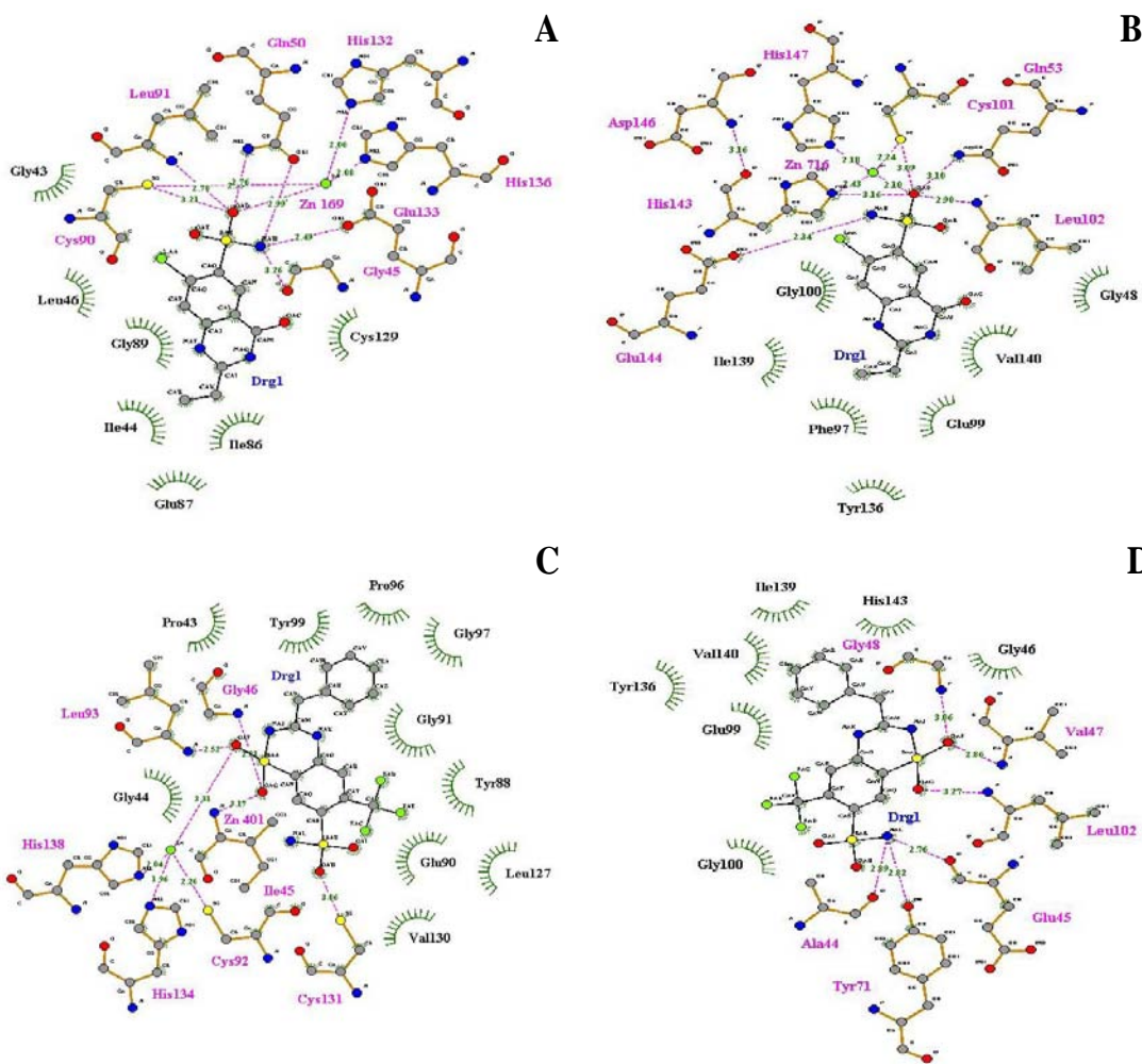
Fig. 3: Molecular interaction pattern of Thiazides with Peptide Deformylase protein models. A) DB01325 with 1BSK, B) DB01325 with 1SZZ, C) CID_6604206 with 1N5N and D) CID_6604206 with 1SZZ
