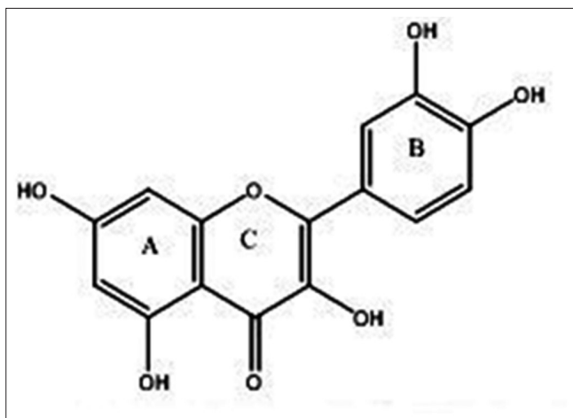
Fig. 5: Flavonoid
