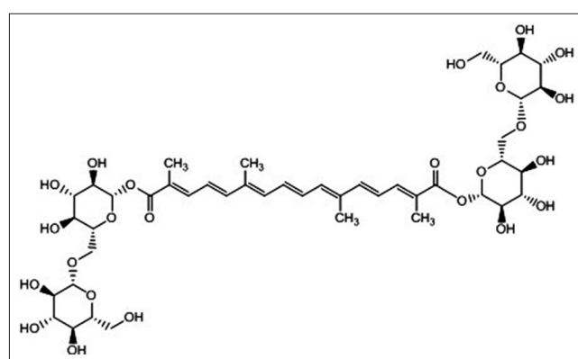
Fig. 9: Crocin
