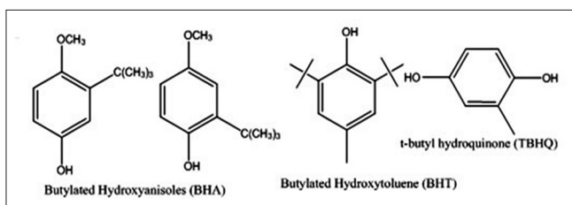
Fig. 4: Synthetic antioxidants
