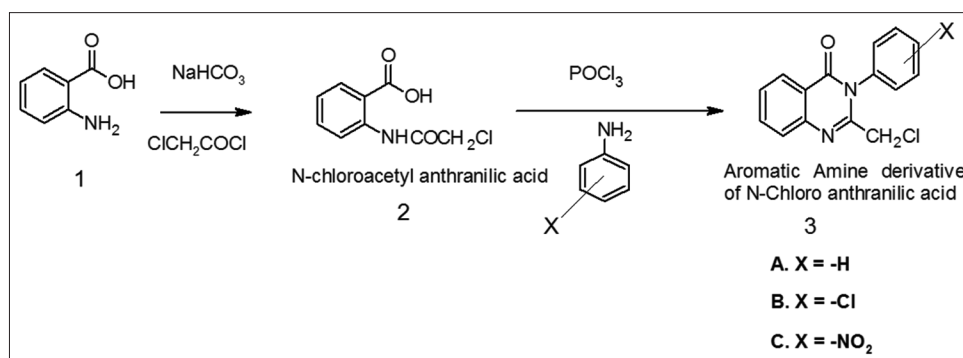
Scheme 1: Preparation procedure of different aromatic amine derivatives of N-chloro anthranilic acid
