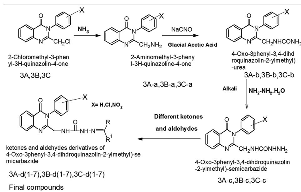
Scheme 2: Preparation procedure of quinazolinone semicarbazone derivatives
