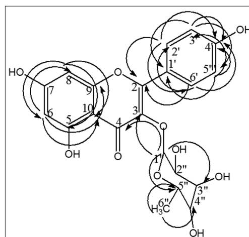
Fig. 1: Heteronuclear single quantum coherence and heteronuclear multiple bond correlation of compound R
