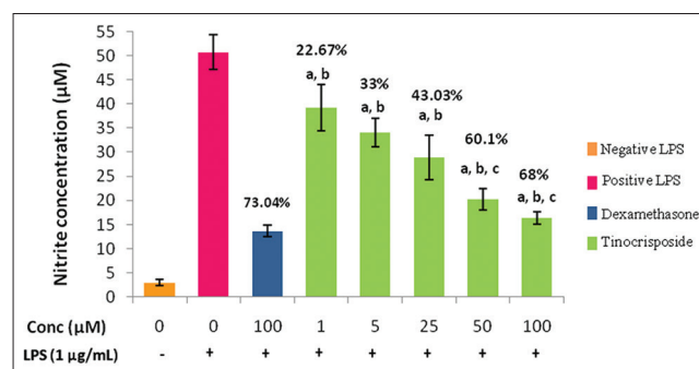
Fig. 3: Effect of tinocrisposide on the nitric oxide production in lipopolysaccharides (LPS)-stimulated cells. Cells were pre-incubated with compound for 1 h and then incubated with LPS for 15 h at 37°C in humidified atmosphere containing 5% \text{CO}_2 . Error bars represent the standard deviation of triplicate values.
