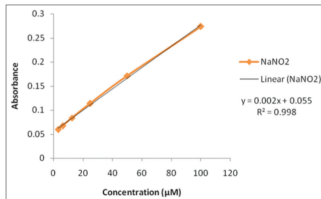
Fig. 2: Calibration curve of nitrite solution
