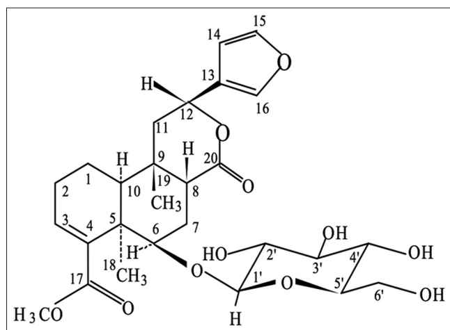
Fig. 1: Chemical structure of tinocrisposide [8]
