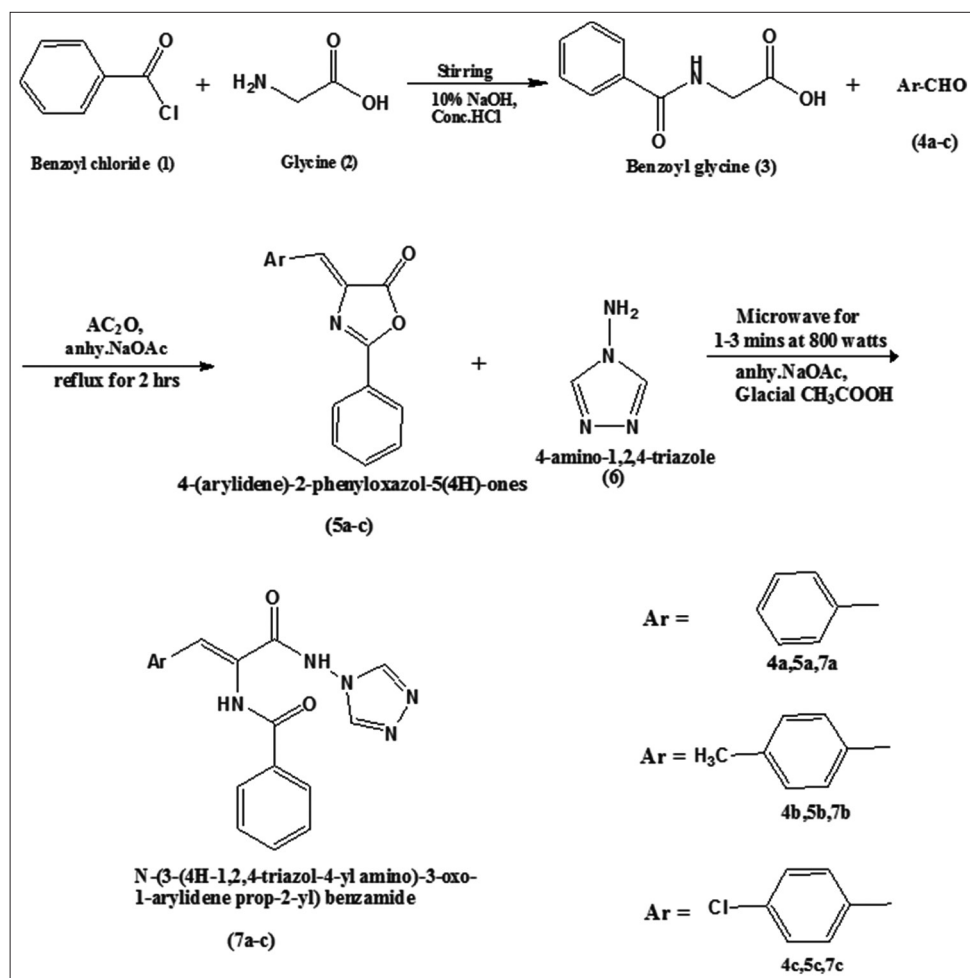
Fig. 1: Synthesis of final compounds (7a-c)
