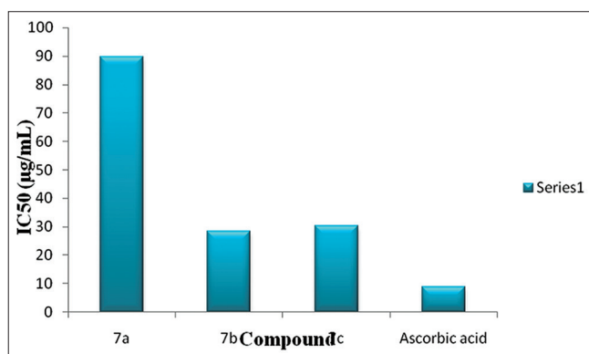
Fig. 4: Graphical representation of antioxidant activity of 7a-c by 2, 2-diphenyl-1-picrylhydrazyl free radical scavenging method
