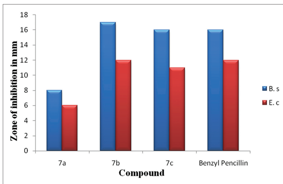
Fig. 2: Graphical representation of antimicrobial activity of 7a-c by paper disc method
