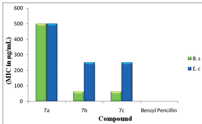
Fig. 3: Graphical representation of antimicrobial activity of 7a-c by microdilution method
