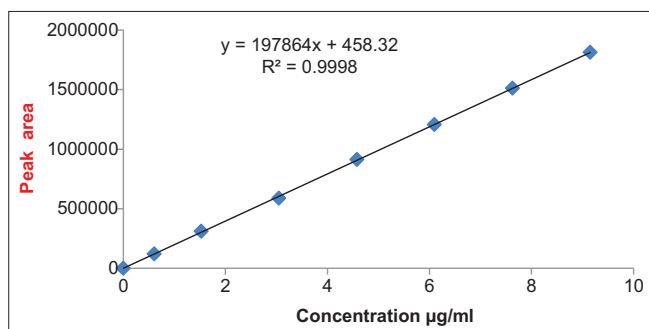
Fig. 4: Linearity curve of nateglinide
