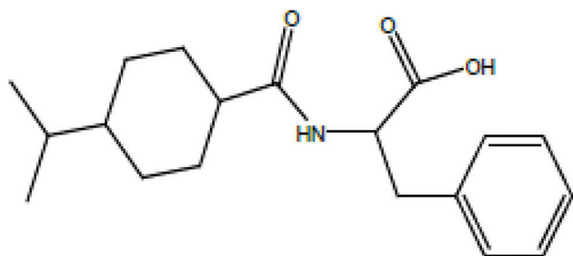
Fig. 1: Chemical structure of nateglinide
