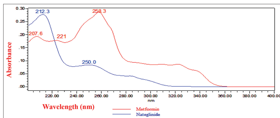
Fig. 3: Selection of isosbestic point for nateglinide and metformin HCl
