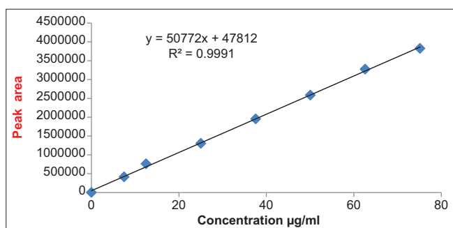
Fig. 5: Linearity curve of metformin HCl
