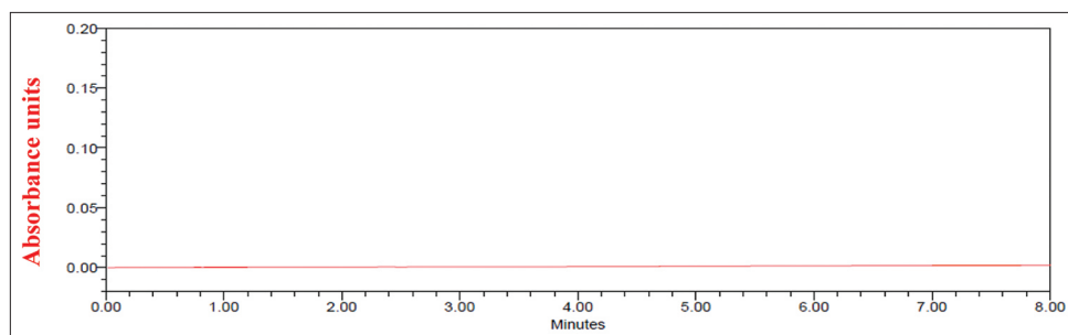
Fig. 7: Chromatogram of placebo
