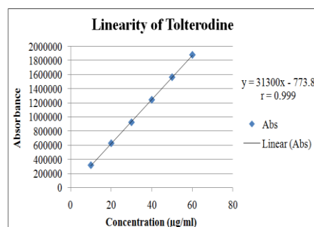
Fig .3: Linearity of Tolterodine in the range 10 to 60 µg/ml.
