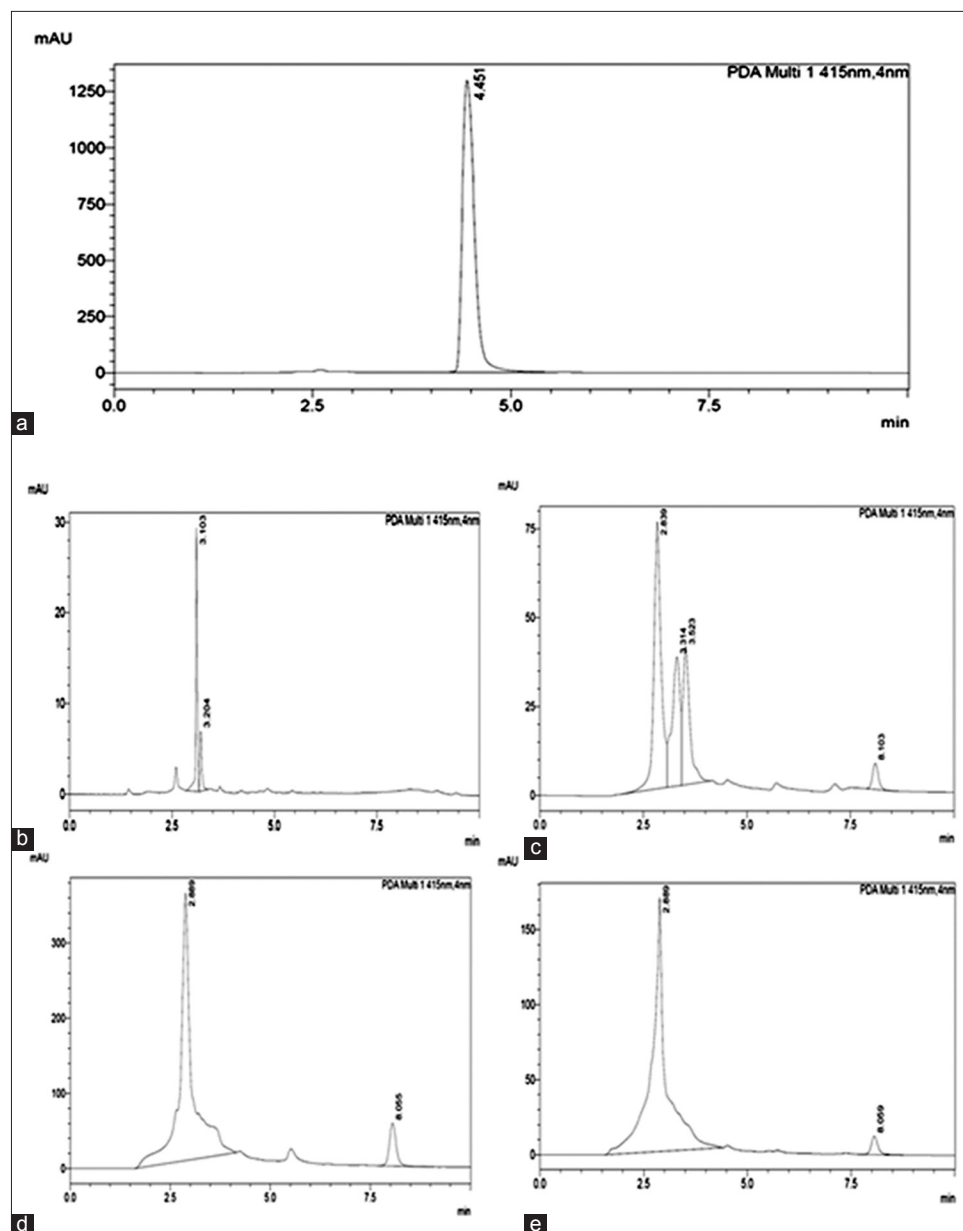
Fig. 3: High performance liquid chromatography chromatogram of (a) Quercetin as a standard of flavonoids, (b) flower anthers, (c) petals, (d) fruit pulp, and (e) rind
