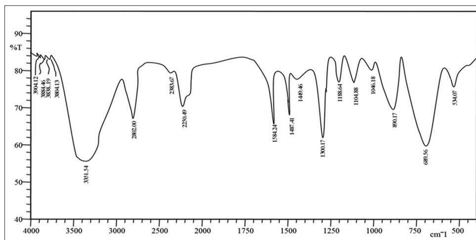
Fig. 2: Fourier transform infrared spectroscopy of infrared-poly lactic-co-glycolic acid nanoparticles
