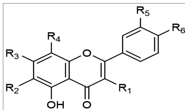
Fig.1: Phenolic compounds isolated from S. montana L.
