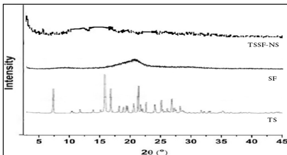
Fig. 6: (a) XRD of Telmisartan, (b) XRD of Silk Fibroin, and (c) XRD of Silk Fibroin nanospheres TSSF-NS5 using X-ray diffractometer (Rigaku Ultima III, Rigaku Corporation) 2\theta range of 0^{\circ} to 45^{\circ}
