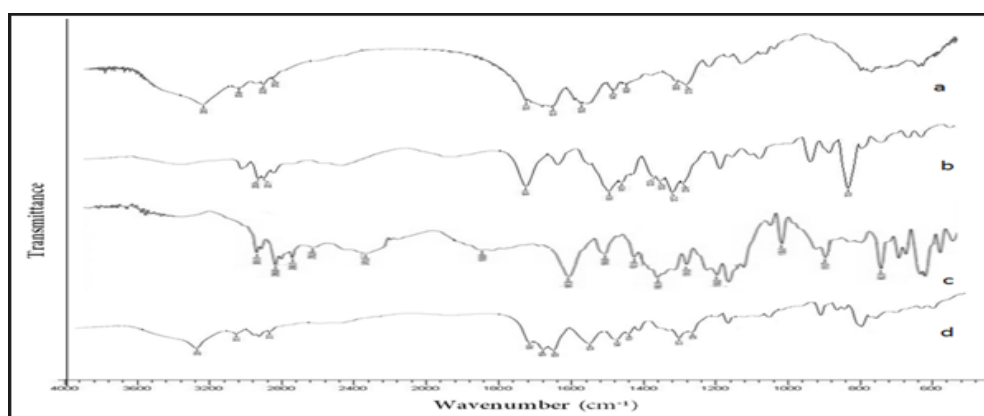
Fig. 4: (a) FTIR of Pure drug telmisartan, (b) FTIR of silk fibroin, (c) FTIR physical mixture of pure drug and polymer, and (d) FTIR of telmisartan nanosphere TSSF-NS5 by using FTIR-spectrophotometer shimadzu-8400 (scan range from 600-4000 \text{cm}^{-1} )
