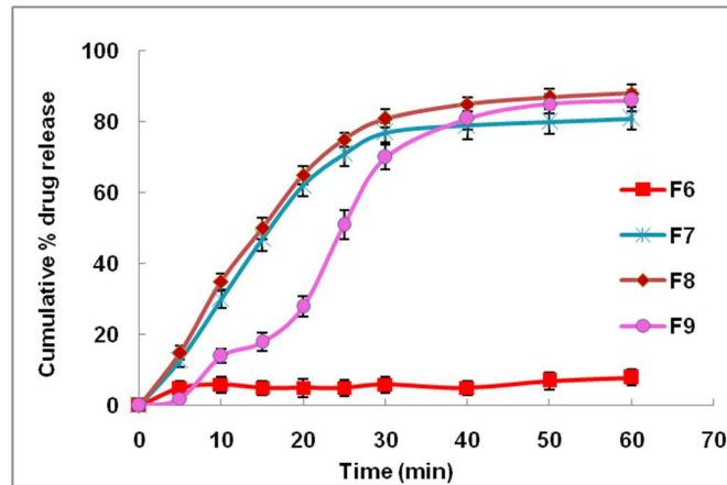
Fig. 5: Effect of type of suppository bases on the in vitro release of piroxicam from hollow suppositories containing piroxicam powder in their cavities using phosphate buffer pH 7.4 at 37°C. [F6 (Witepsol H 35), F7 (PEGs 200:6000 70:30), F8 (PEGs 400:4000 70:30) and F9 (Glycerinated gelatin base)]
