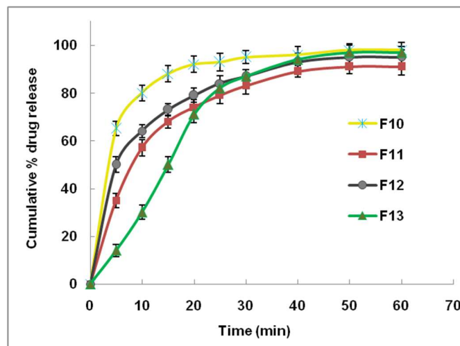
Fig. 6: Effect of type of suppository base on the in vitro release of piroxicam from hollow suppositories containing piroxicam solution in their cavities using phosphate buffer pH 7.4 at 37°C. [F10 (Witepsol H35), F11 (PEGs 200:6000 70:30), F12 (PEGs 400:4000 70:30) and F13 (glycerinated gelatin base)]
