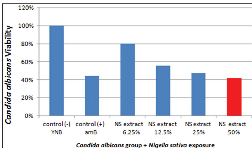
Fig. 2: The percentage of viable Candida albicans cells after Nigella sativa seed extract exposure
