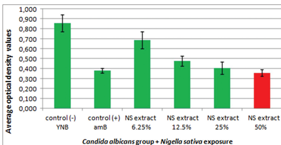
Fig. 1: The average optical density 490 value of Candida albicans after incubation with various concentrations of Nigella sativa seed extract at 37°C for 24 h
