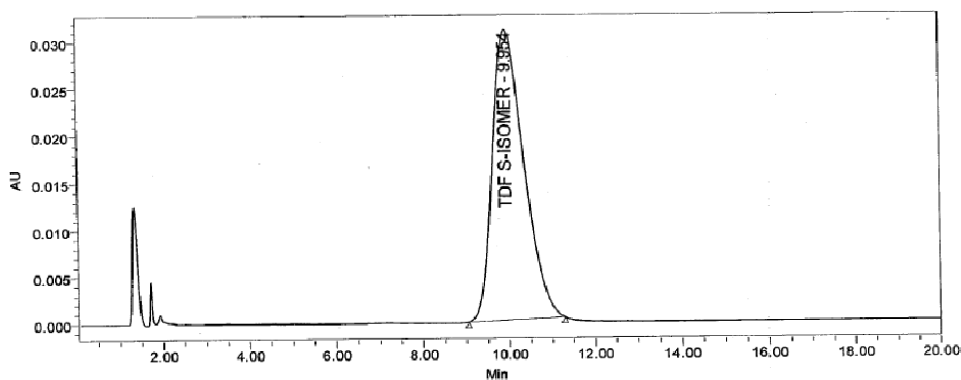
Fig. 5: (S) Isomer 0.1 mg/ml solution
