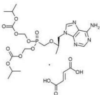
Fig. 1: Chemical structure of tenofovir disoproxil fumarate
