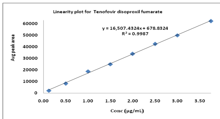
Fig. 6: Linearity plot for tenofovir disoproxil fumarate
