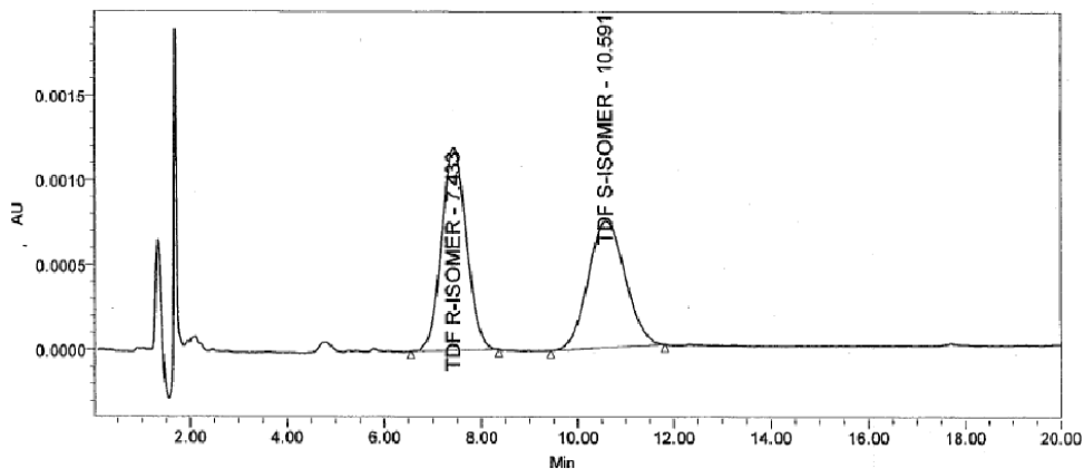
Fig. 3: Tenofovir disoproxil fumarate and (S) enantiomer
