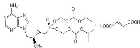
Fig. 2: Chemical structure of tenofovir disoproxil fumarate (S) enantiomer
