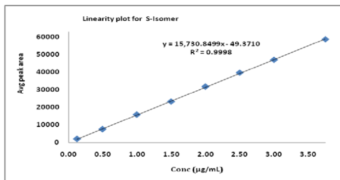
Fig. 7: Linearity plot for S-Isomer
