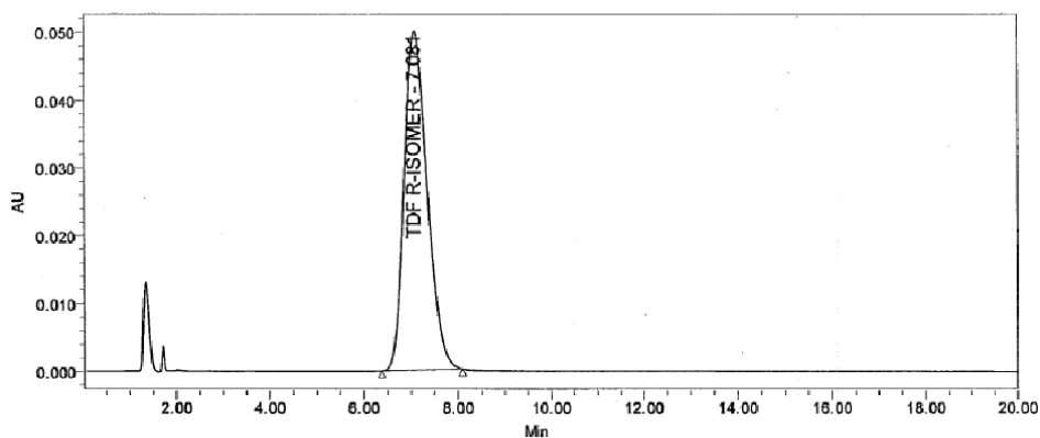
Fig. 4: Tenofovir disoproxil fumarate 0.1 mg/ml solution
