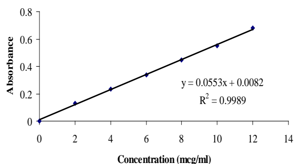
Fig. 1: Calibration curve of tizanidine hydrochloride in pH 1.2 buffer
