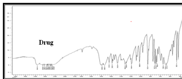
Fig. 3: FTIR data of pure drug
