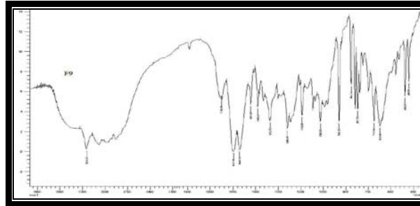
Fig. 4: FTIR spectra of formulations F2, F4, F6, F8 and F9
