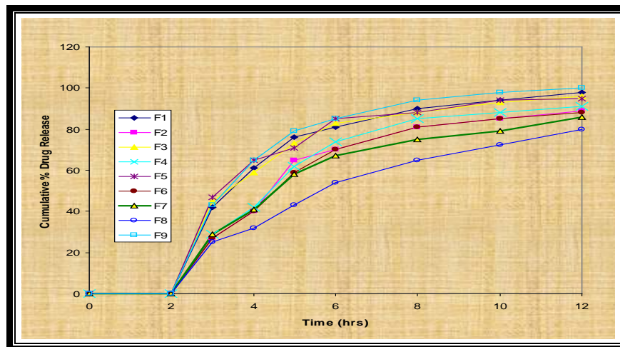
Fig. 6: In vitro release pattern for the prepared formulations
