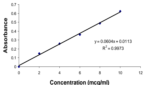
Fig. 2: Calibration curve of tizanidine hydrochloride in pH 7.4 phosphate buffer
