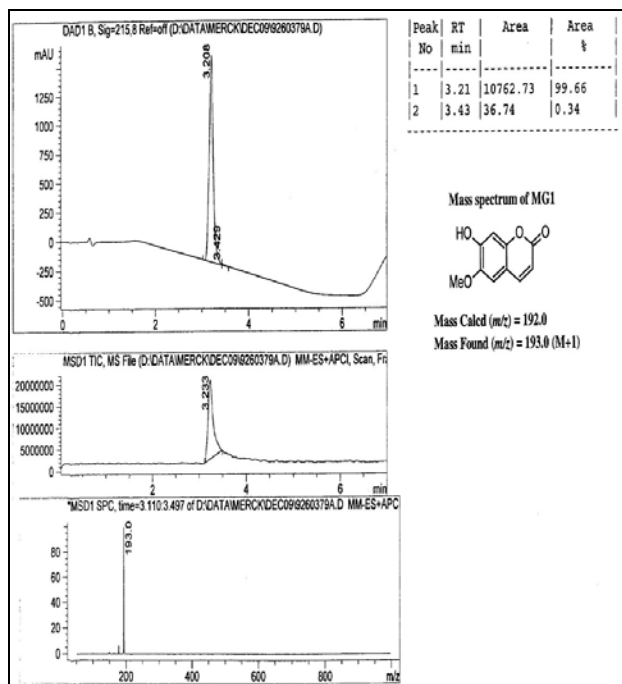
Fig. 2: Mass Spectrum of MG1
