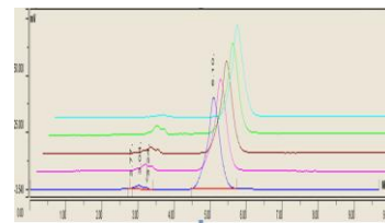
Fig 1:Chromatogram of standard Donepezil HCl
