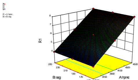
Fig. 6: 3D response surface graph for lag time
