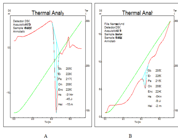
Fig. 3: DSC thermogram of: A) Acebrophylline B) Acebrophylline + excipients
