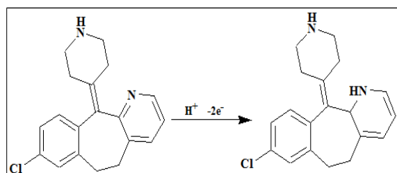
Scheme 1: Reduction mechanism of DLTD
