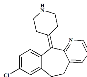
Fig. 1: Structure of desloratadine (DLTD)
