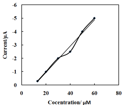
Fig. 7: Calibration plot of the DLTD in PB solution pH, at different concentrations at glassy carbon electrode
