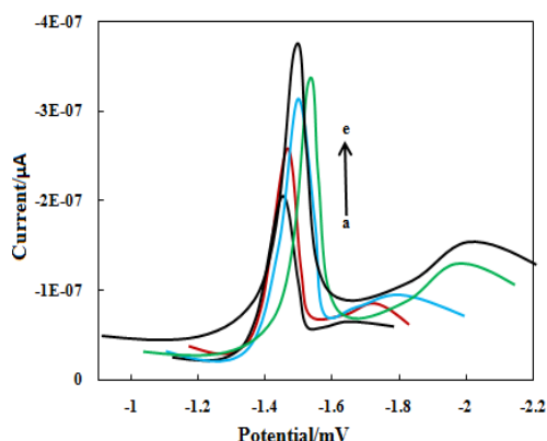
Fig. 6: Typical square wave voltammograms of DLTD in PB solution pH 9.0, concentration: 1.0 \times 10^{-3} \text{M} to 2.55 \times 10^{-5} \text{M} (a to e) at glassy carbon electrode
