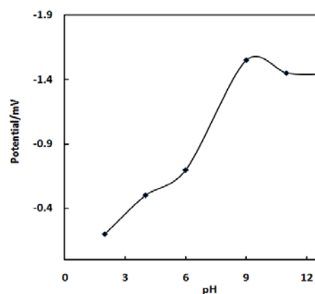
Fig. 4: The plot of the potential vs pH of DLTD in PB solution, concentration: 2.55 \times 10^{-5} M at glassy carbon electrode in different pH values.
