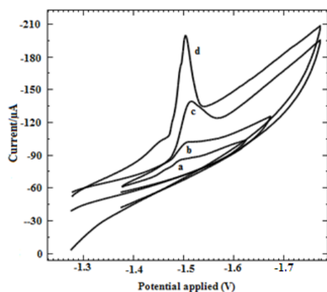
Fig. 2: Typical cyclic voltammograms of DLTD in PB solution, concentration: 2.55 \times 10^{-5} M at glassy carbon electrode in different pH values from pH 4.0-10.0 (a to d)
