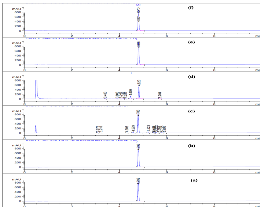
Fig. 4: (a) Typical chromatogram of carvedilol under stress conditions: (a) thermal degradation, (b) photolytic degradation, (c) acid hydrolysis, (d) oxidative degradation, (e) base hydrolysis and (f) in water
