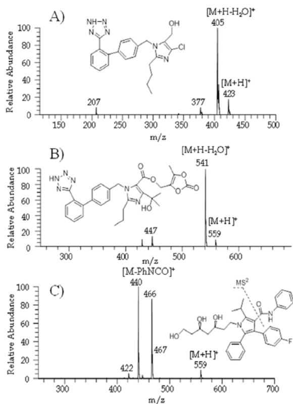
Fig. 1: LC-ESI-MS/MS spectra of A) losartan, B) olmesartan and C) atorvastatin and their corresponding structures
