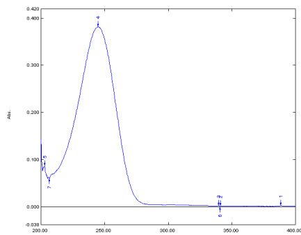
Fig. 2: UV spectrum of standard
