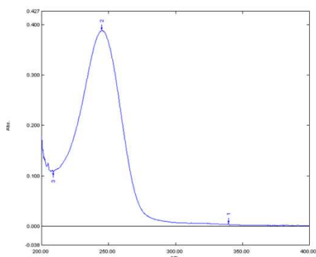
Fig. 3: UV spectrum of sample
