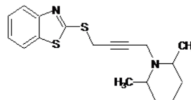
Fig. 4: Synthesis of 2-[[4-(2,6-dimethylpiperidin-1-yl)but-2-yn-1-yl]sulfanyl]-1,3-benzothiazole (AZ3)
