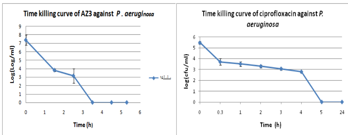
Fig. 5: Time exposure viability curve for addition of compound AZ3 and ciprofloxacin, at MBC (250 µg/ml) to culture of P. aeruginosa ATCC 9027
