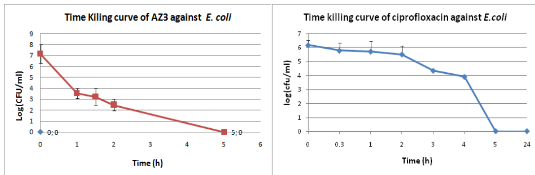
Fig. 6: Time exposure viability curve for addition of compound AZ3 and ciprofloxacin, at MBC (500 µg/ml) and (125 µg/ml) respectively to culture of E. coli ATCC 8739
