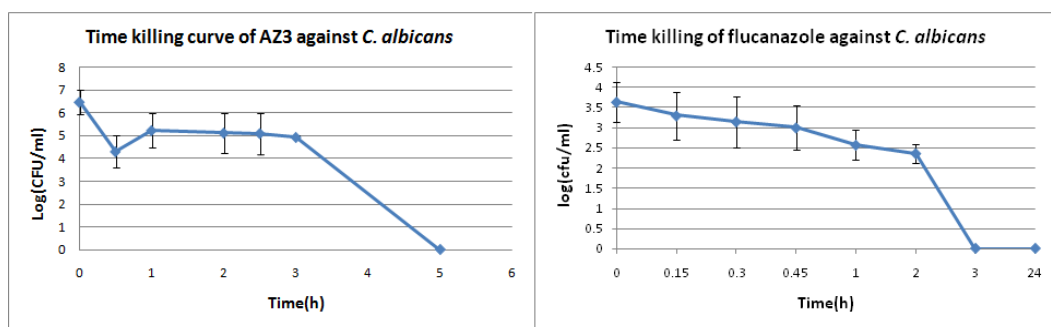
Fig. 9: Time exposure viability curve for addition of compound AZ3 and fluconazole, at MFC (250 µg/ml) and (500 µg/ml) respectively to culture of C. albicans ATCC 10231
