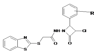
Fig. 1: 4-substituted phenyl-3-chloro-1-[(benzothiazolythio)acetamidyl]-2-azetidinone derivatives [8]
