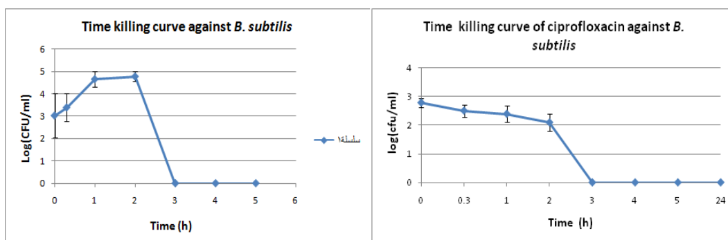
Fig. 8: Time exposure viability curve for addition of compound AZ3 and ciprofloxacin, at MBC (125 µg/ml) and (250 µg/ml) respectively to culture of B. subtilis ATCC 6633
