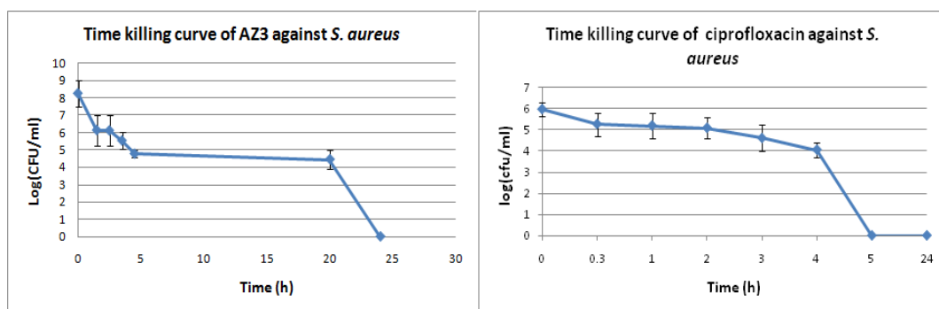
Fig. 7: Time exposure viability curve for addition of compound AZ3 and ciprofloxacin at MBC (250 µg/ml) to culture of S. aureus ATCC 6538
