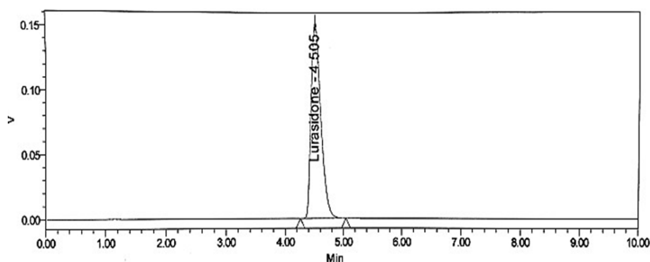
Fig. 2: Optimized chromatogram of standard lurasidone hydrochloride
