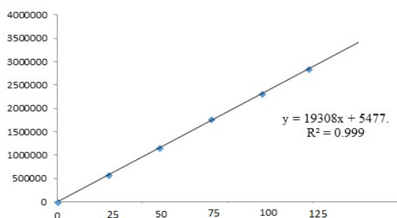
Fig. 4: Linearity plot of lurasidone hydrochloride
