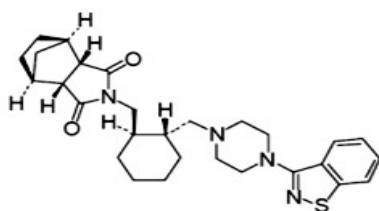
Fig. 1: Chemical structure of lurasidone
