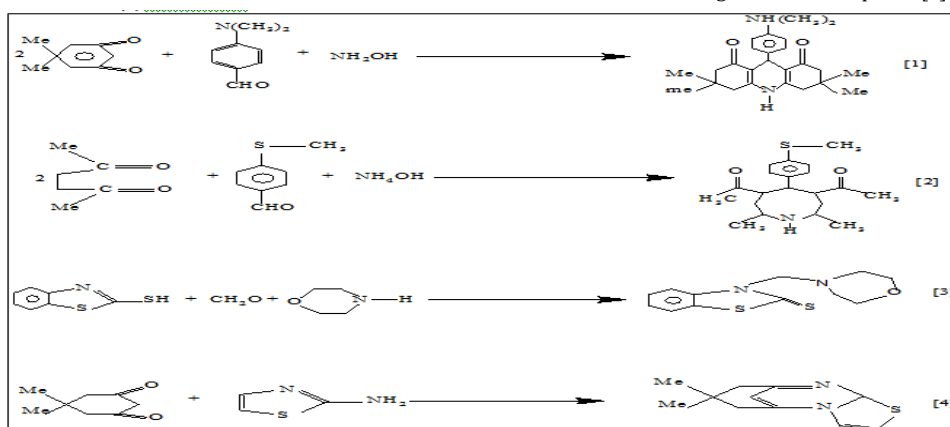
Scheme1: Reactions scheme
