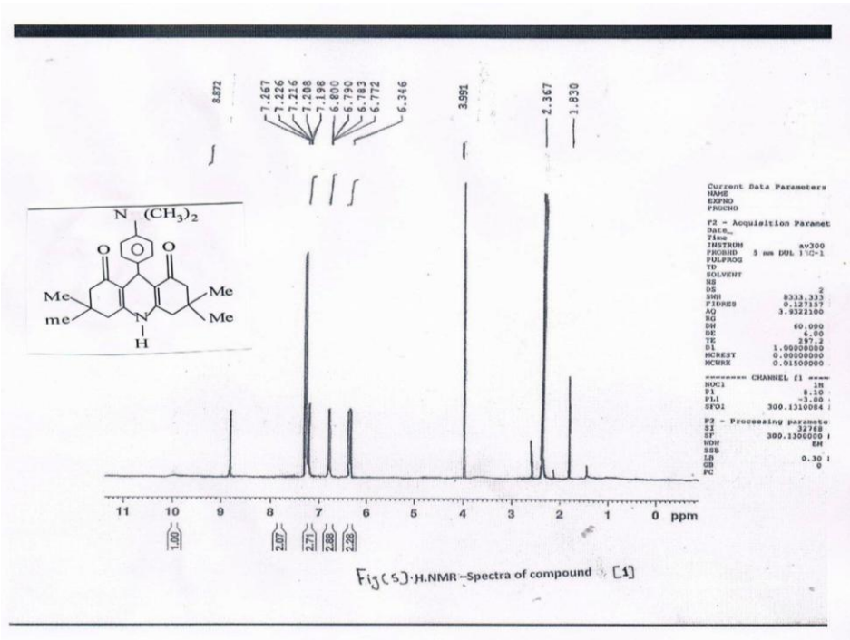
Fig3:1HNMR spectrum of Compound[1]
