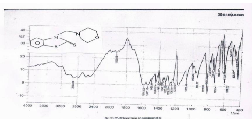
Fig (3) FT-IR Spectrum of compound[3]
