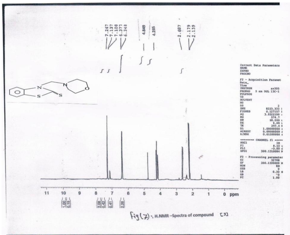
Fig5:1HNMR spectrum of Compound[3]
